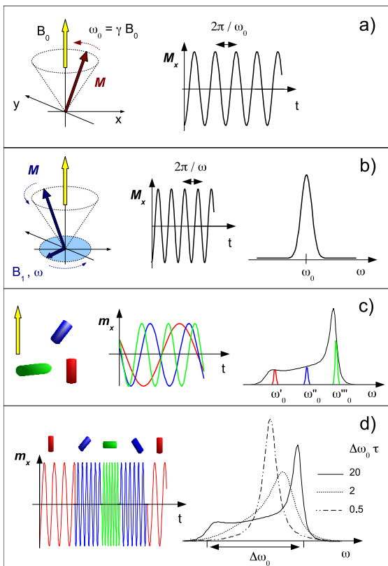
Fig. 1. Aspects of the ESR spectroscopy. a) free precession of the magnetization M of an ensemble of isolated electrons around the static magnetic field B_0 with Larmor angular frequency \omega_0 = \gamma B_0 , \gamma being the magnetogyric ratio. The transverse magnetization oscillates at the same frequency. b) In condensed matter the electrons exchange energy with the surroundings. A rotating microwave field B_1(t) \perp B_0 with angular frequency \omega forces the precession of the magnetization around B_0 with the same angular frequency. When \omega \simeq \omega_0 an absorption resonance occurs. c) The magnetic dipoles m of immobile spin probes in a frozen liquid have different \omega_0 values due to their different orientations with respect to B_0 , thus resulting in a broad line with width \Delta\omega_0 (black line), usually referred to as rigid-limit or powder lineshape. d) If the spin probe undergoes rotation (sketched as instantaneous clockwise jumps at random times), \omega_0 fluctuates. When the rotational rate 1/\tau is larger than the width of the \omega_0 distribution \Delta\omega_0 , the different precession frequencies become indistinguishable and an average value is seen, i.e. the ESR lineshape coalesces (motional narrowing).
