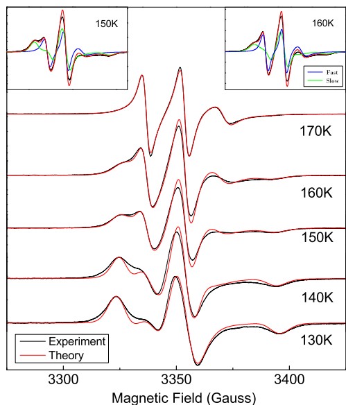
Fig. 3. ESR lineshapes of TEMPOL in DH regime. Note the growth of the narrow component (fast TEMPOL) which superimposes to the broader one (slow TEMPOL) with increasing temperature. The insets show the fast (blue) and slow (green) components of the overall lineshape (red) at two temperatures.
