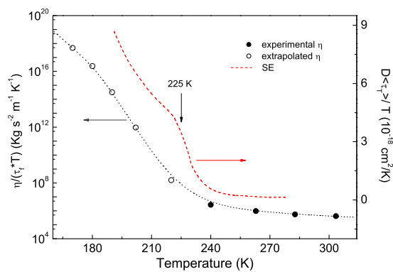
Fig. 5. Breakdown of the DSE law. Data are compared with the SE breakdown from ref.[18]. Filled dots refer to temperatures where experimental values of the viscosity are available. Empty dots are based on a thermodynamic extrapolation of the viscosity [39]. The line across the dots is a guide for the eyes.
