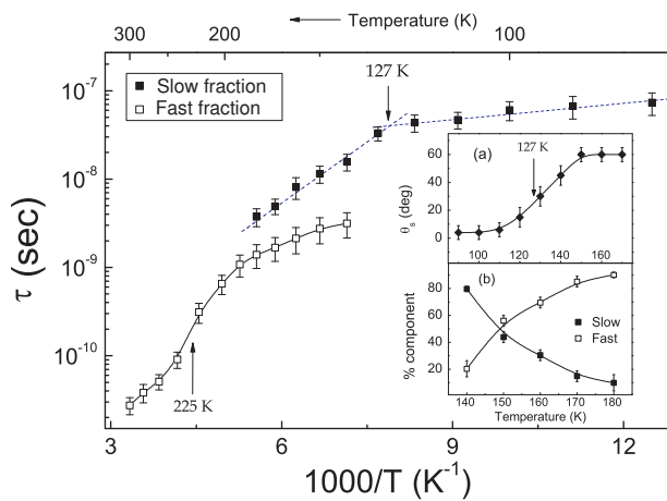
Fig. 4. Temperature dependence of the rotational parameters of the fast (F) and the slow (S) fractions of TEMPOL in deeply supercooled bulk water. Main panel: rotational correlation times \tau_s and \tau_f . Inset a: average jump angle of the S fraction. Inset b: weights of the F and S fractions. Note in the main panel : i) the knee at \sim 127K close to T_g = 136K , ii) the DH regime ( 140 - 180K ) where the two coexisting TEMPOL fractions with different mobilities are evidenced, iii) the inflection close to T_{FSC} \sim 228K .
