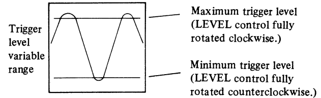
(a) Input signal of large amplitude
