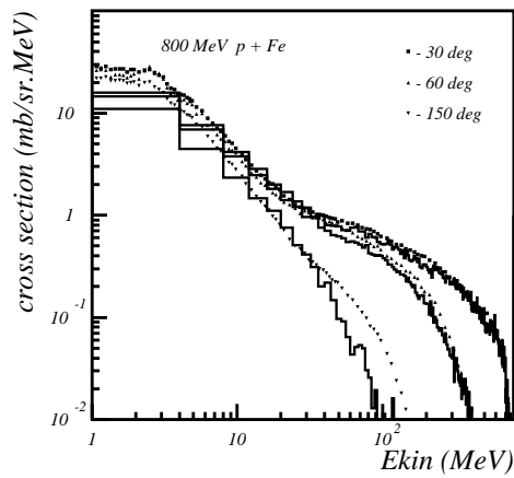
Figure 26.8: Double differential cross-section for neutrons produced in proton scattering off Iron. Proton incident energy was 800 MeV. The points are data, the histogram is Binary Cascade prediction.
