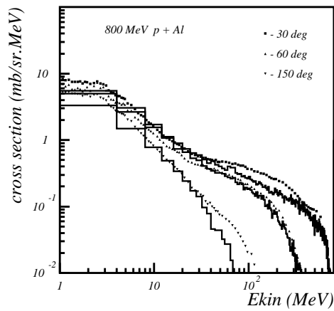
Figure 26.4: Double differential cross-section for neutrons produced in proton scattering off Aluminum. Proton incident energy was 800 MeV. The points are data, the histogram is Binary Cascade prediction.
