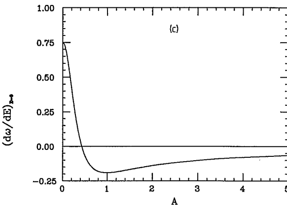
FIG. 1. (a) The dependence of the eigenfrequency \omega(E) of the oscillations on the energy E of the oscillator, measured from the bottom of the potential well, for several values of the inclination parameter A , calculated from Eqs. (4a) and (4b). The corresponding values of A , from bottom to top, were 0, 0.2, 0.43, 0.6, 1.0 and 2.0. (b) As in (a), but over a wider range of E . (c) The dependence on A of the initial gradient \omega'_0 = [d\omega(E)/dE]_{E=0} of the curves shown in (a), calculated from (5) and (6).
