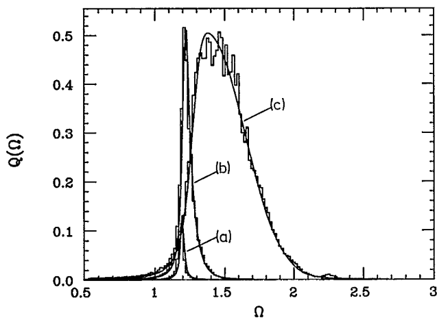
FIG. 3. Spectral density of the fluctuations Q(\Omega) of the oscillator (2) and (7) calculated (solid curves) from (16) and measured (histograms) for the analog electronic model with the inclination parameter A=0.43 for noise intensities: (a) T=0.0191 ; (b) 0.154; (c) 1.15.
