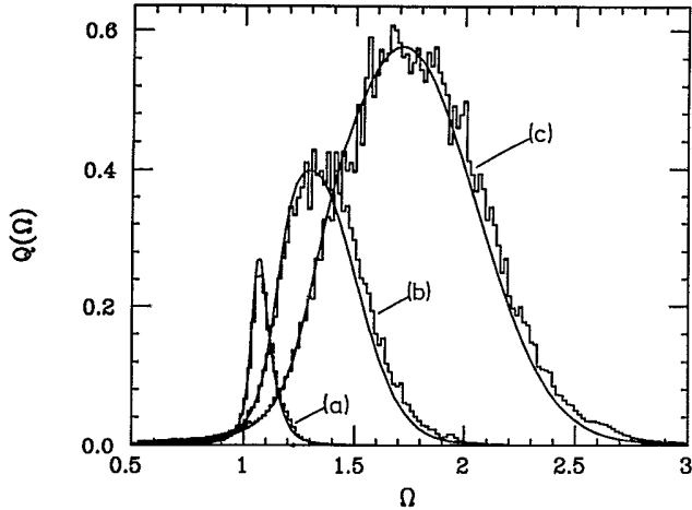
FIG. 2. Spectral density of the fluctuations Q(\Omega) of the oscillator (2) and (7) calculated (solid curves) from (16) and measured (histograms) for the analog electronic model, with the inclination parameter A=0 , for noise intensities: (a) T=0.078 ; (b) 0.687; (c) 3.04.
