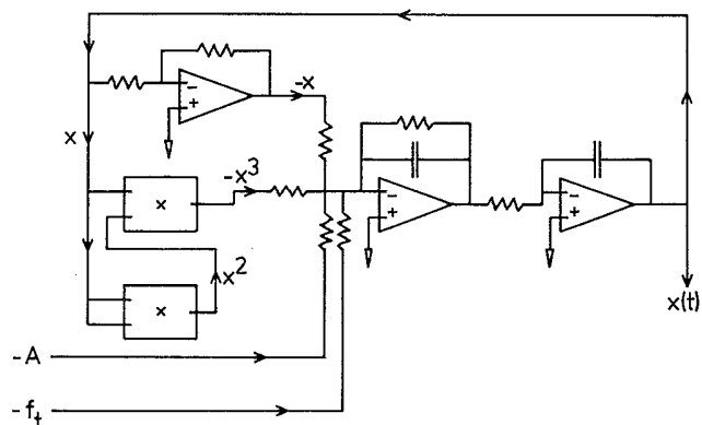
FIG. 5. Block diagram of the circuit used to model the system (2) and (7).
